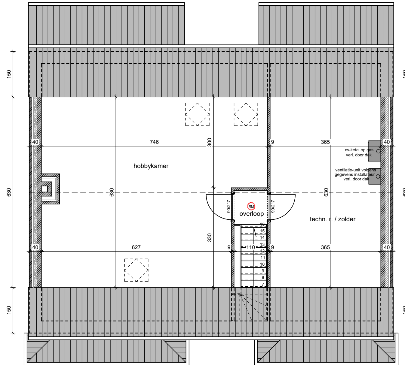
plan zolder
