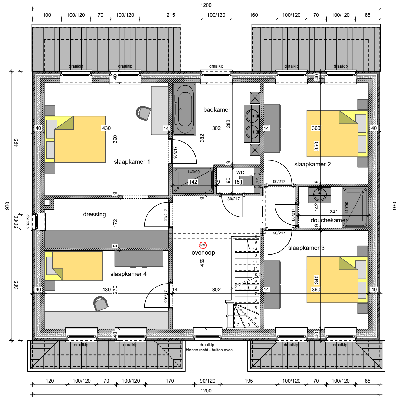
plan verdieping
