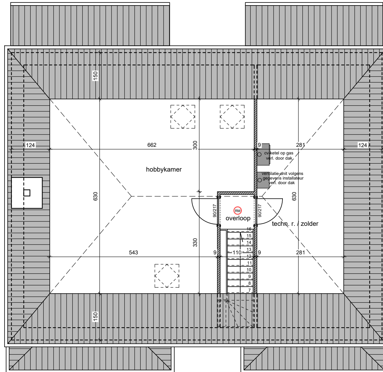
plan zolder
