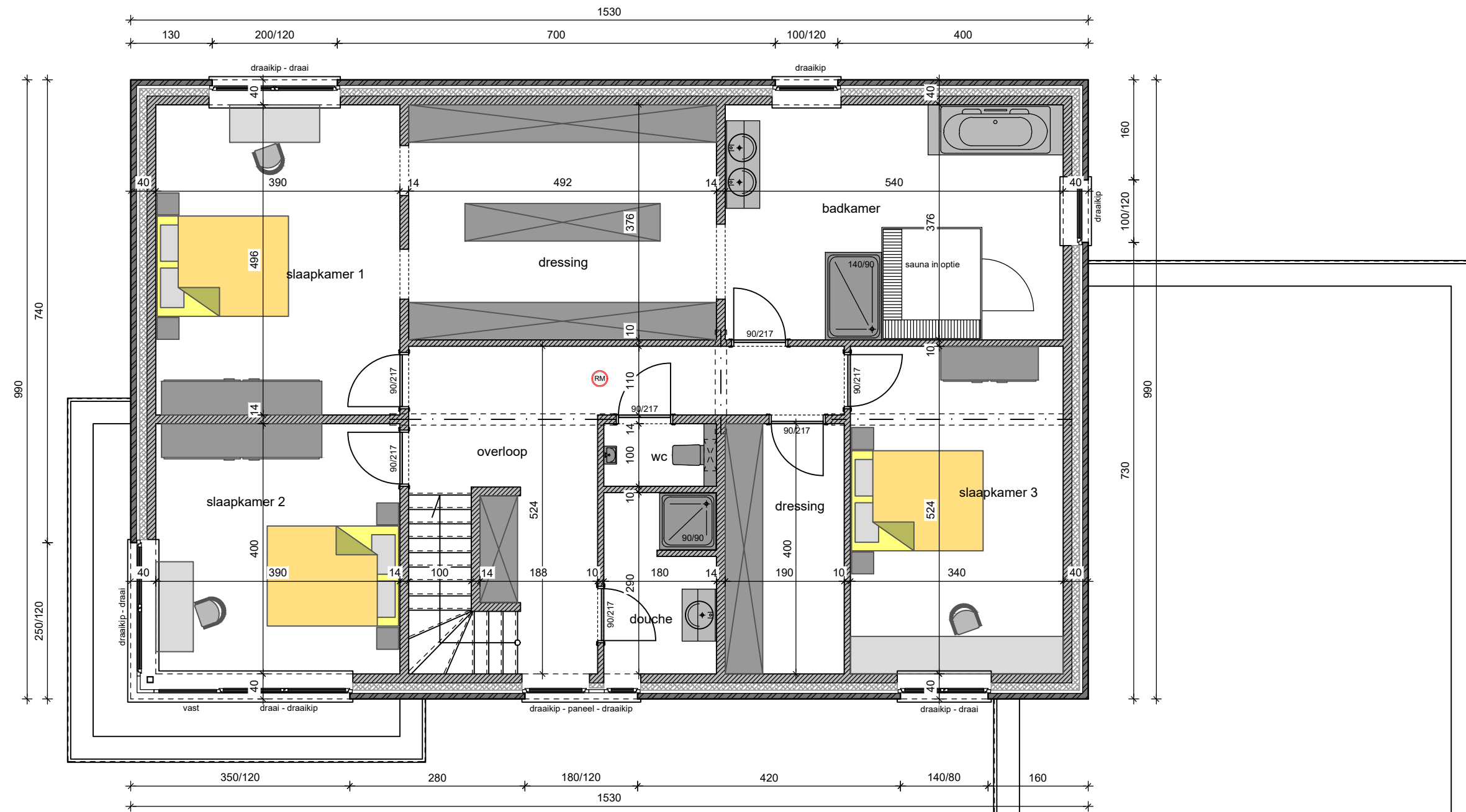
plan verdieping
