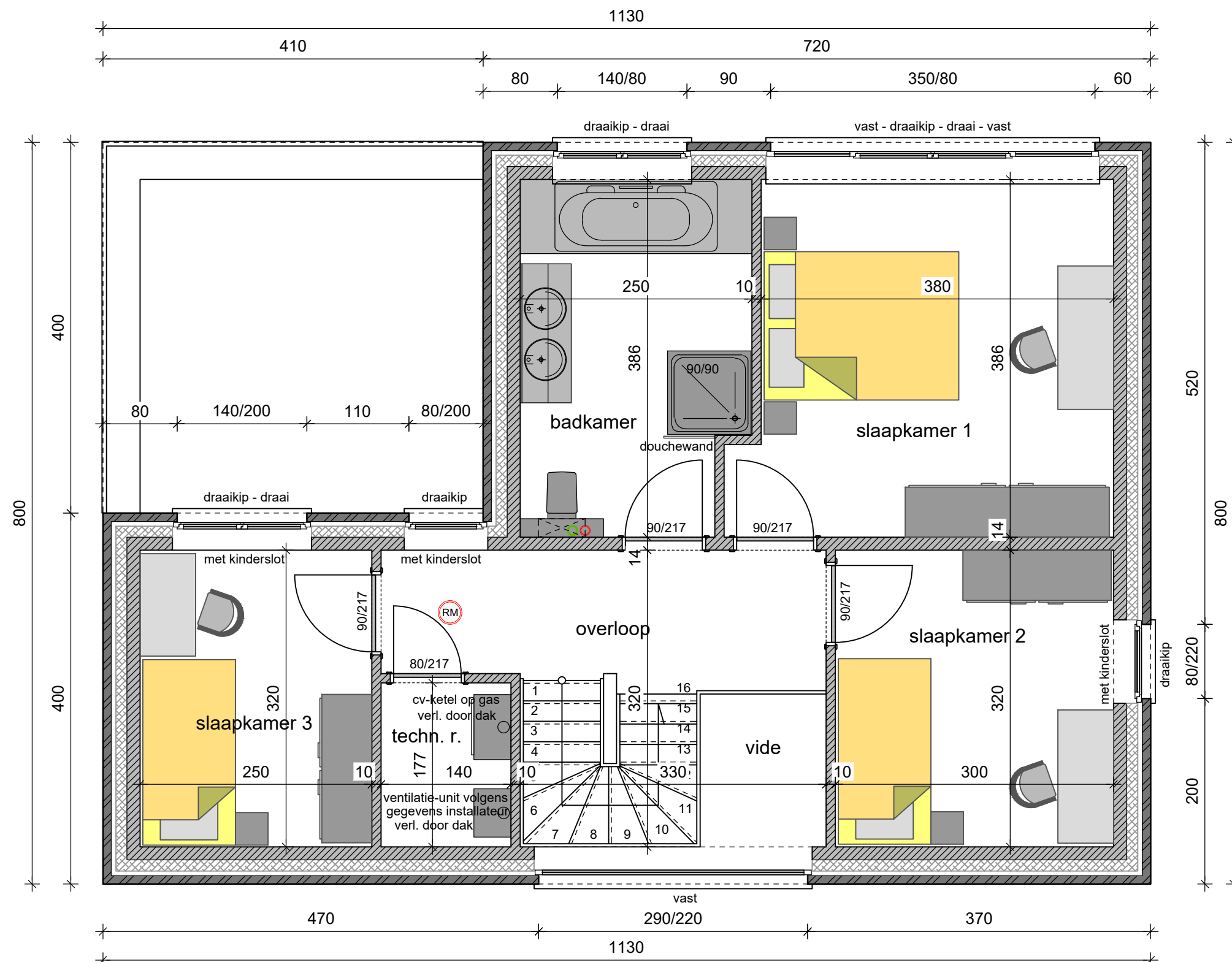
plan verdieping
